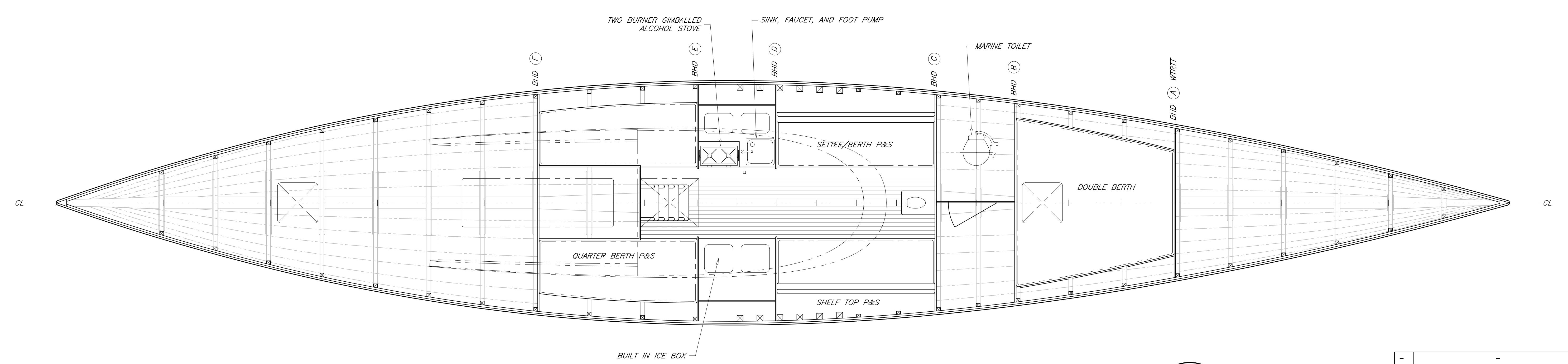
PLAN A-5 BELOW DECK ARRANGEMENT
