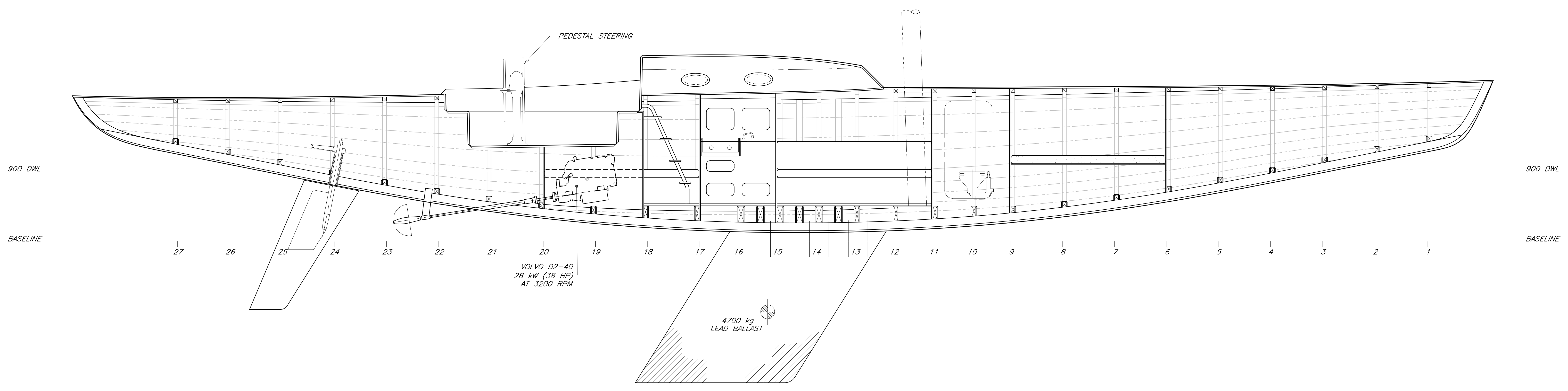
ELEVATION C-5 PORT INBOARD PROFILE
