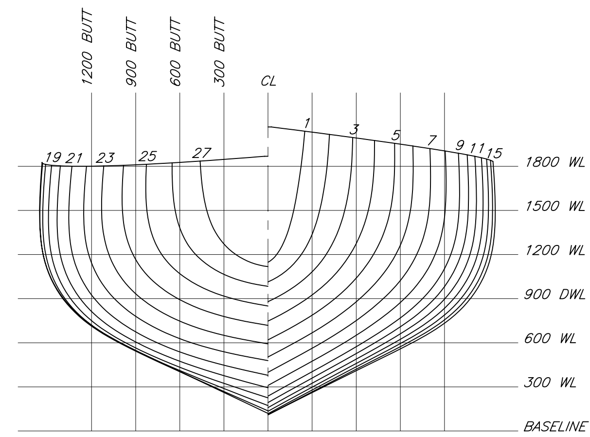
ELEVATION B-3 BODY PLAN
