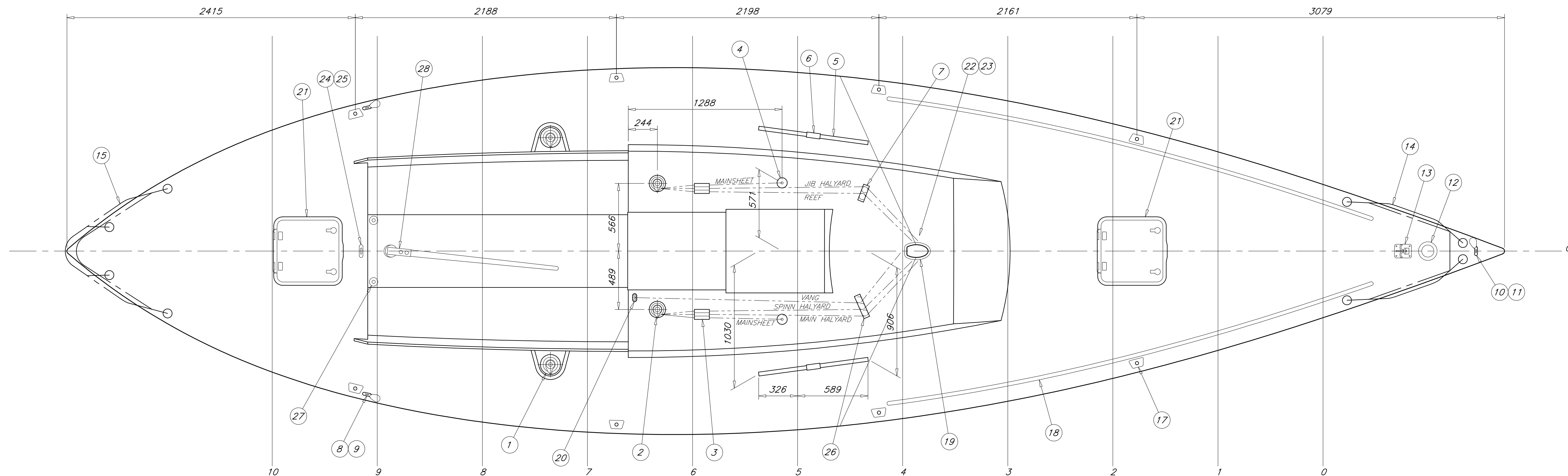
PLAN A-4 DECK PLAN
